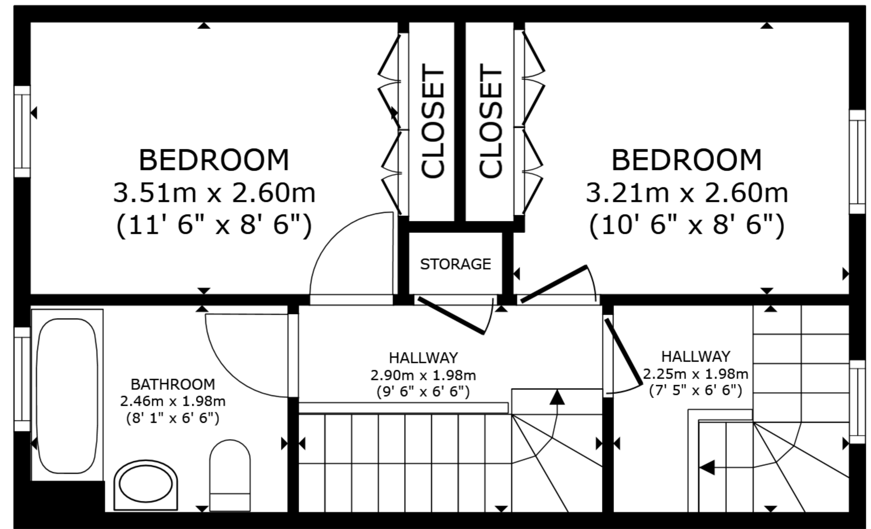
FLOOR 2
